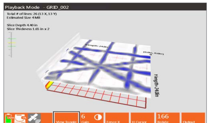
Screen capture of 3D data image. Data illustrates a rebar mat with post tension cables in an “X” pattern.
