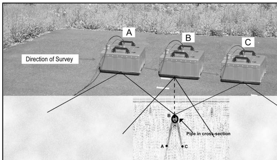
Figure 3: Hyperbola creation.
